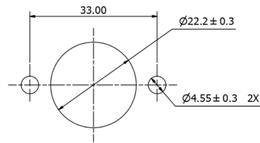
Punched mounting Hole
