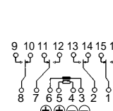
Diagram shows the "reset" position when terminals 3 and 6 are energized. Energize terminals 4 and 5 to transfer contacts.
