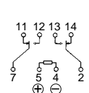
Deenergized position
