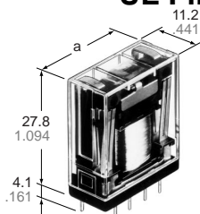
Vertical series (PC board)
