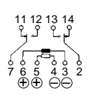
Diagram shows the "reset" position when terminals 3 and 6 are energized. Energize terminals 4 and 5 to transfer contacts.
