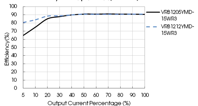
Efficiency Vs Output Load (Vin=12V)
