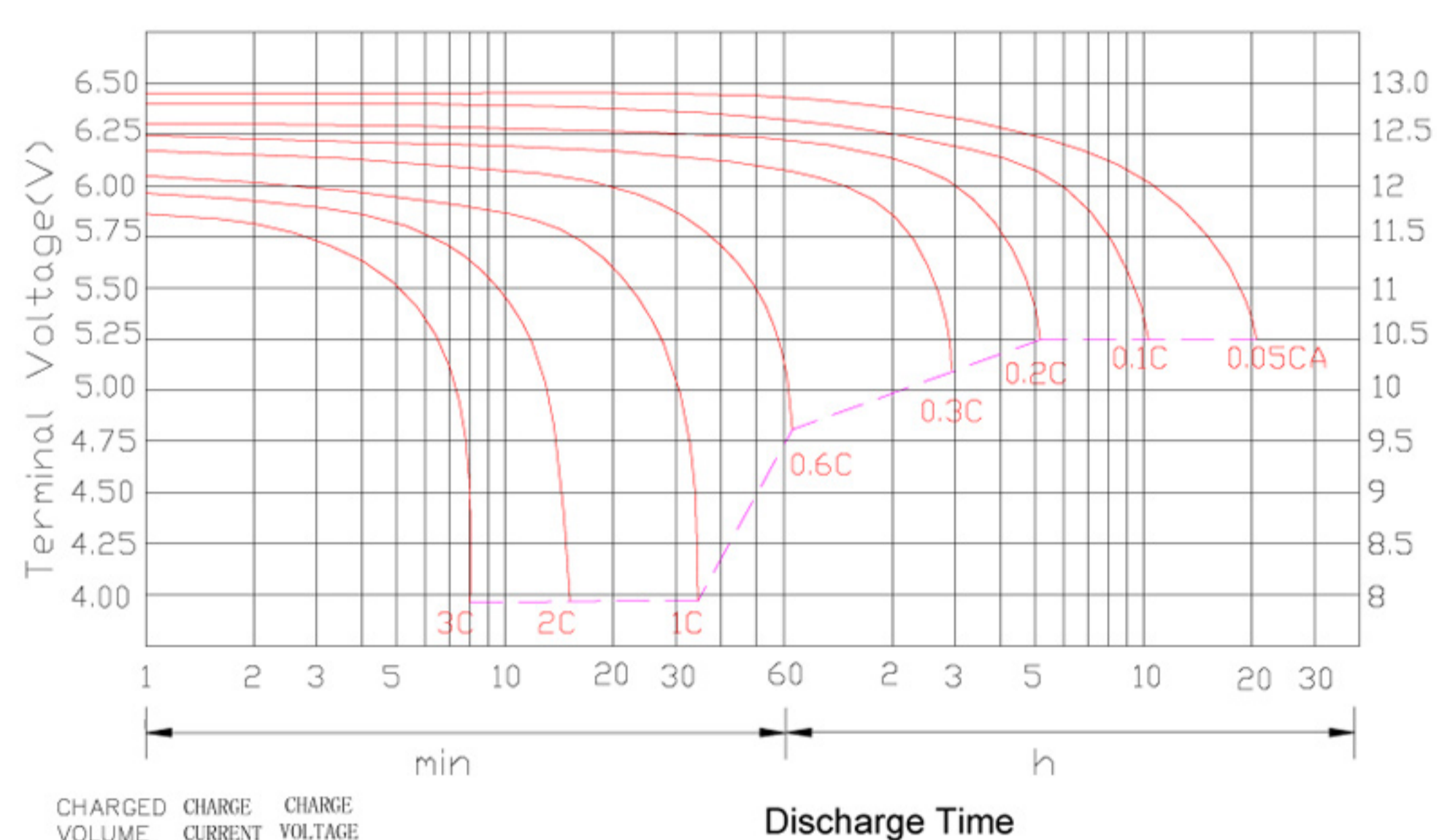
DISCHARGE CHARACTERISTICS AT 25° C(77° F)
