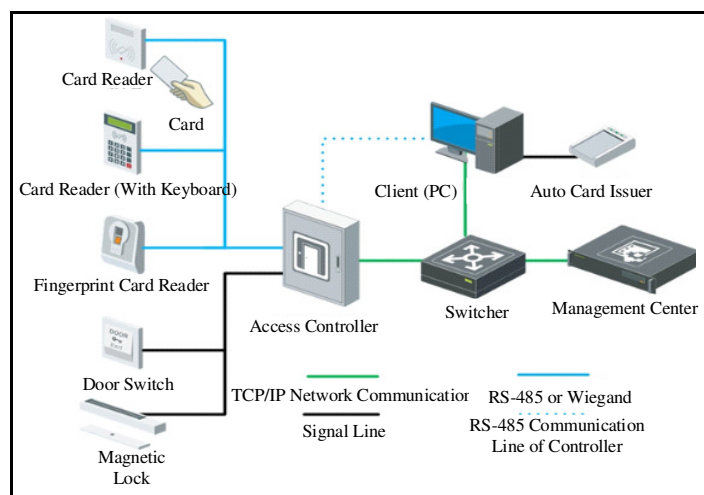
Topological Graph
