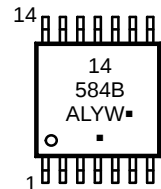
TSSOP-14 DT SUFFIX CASE 948G
