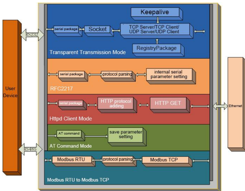
USR-N520 Function Diagram
