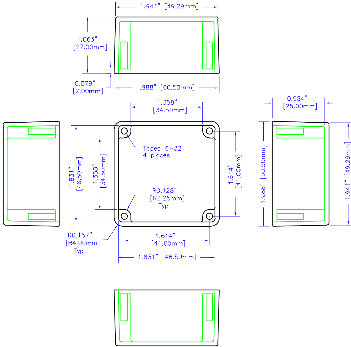
BOX
