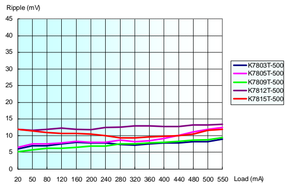
Ripple VS Load (Vin=Normal)
