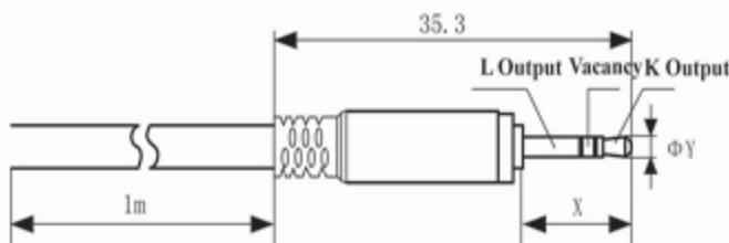
Diagram for standard three-core plug
