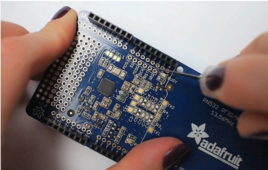
Solder a wire from IRQ to #6
