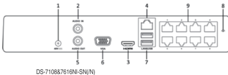
DS-7108&7616NI-SN(/N)
