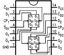
Pin Assignment for DIP, SOIC and TSSOP
