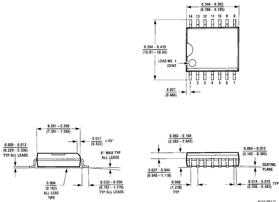
14-Lead Small Outline Integrated Circuit (SOIC), JEDEC MS-013, 0.300mm Wide Body Package Number M14B
