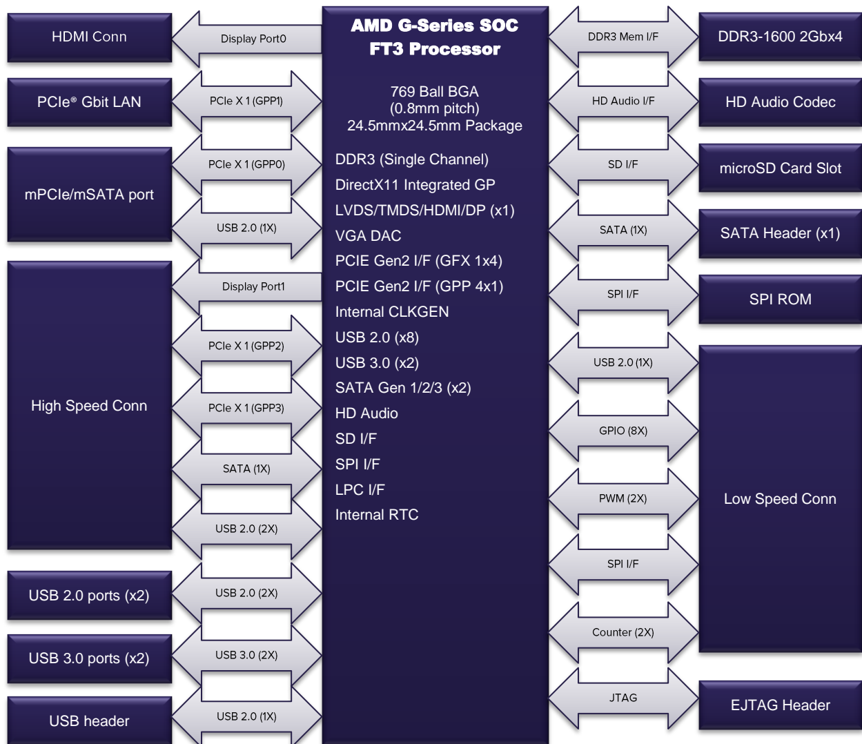
Figure 1 Gizmo 2 Block Diagram
