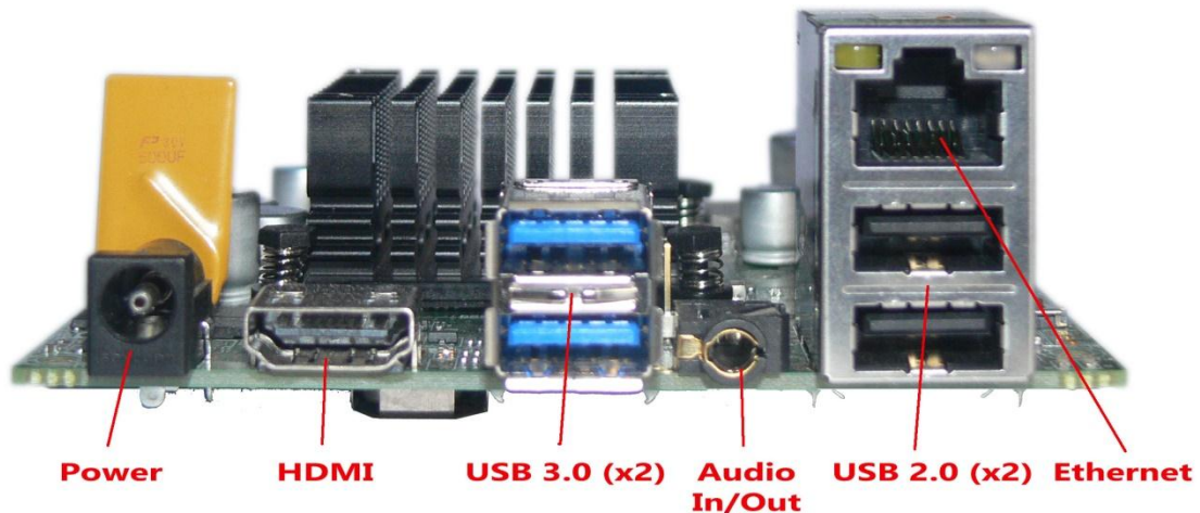
Figure 4 Gizmo 2 Board Back Panel
