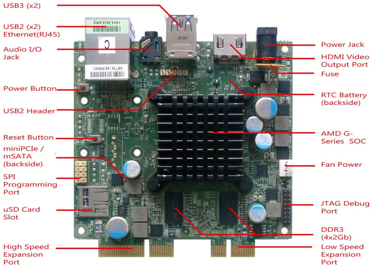
Figure 3 Gizmo 2 Board Connector Locations
