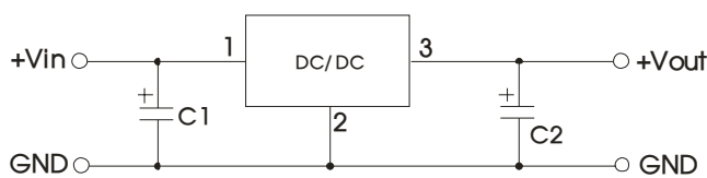
Fig. 2 Positive output application circuit
