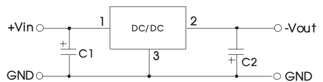
Fig. 3 Negative output application circuit
