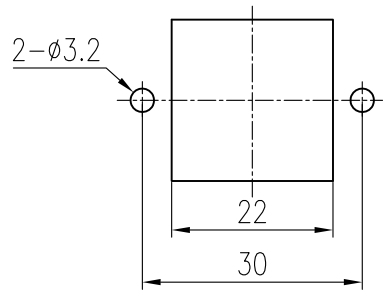
面板开孔图 Panel cut out
