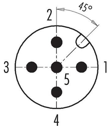
Contact arrangement (Plug-in side)
