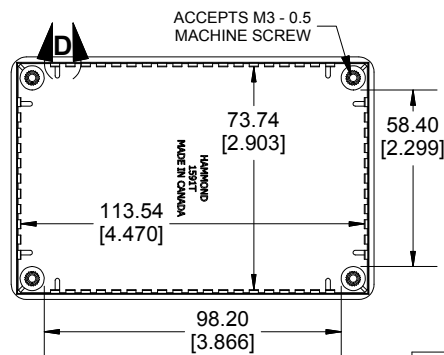
INSIDE BOX
