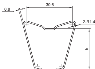
Retainer Dimensions
