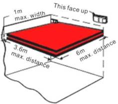
Overhead Curtain
