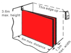
Wall-Mount Curtain
