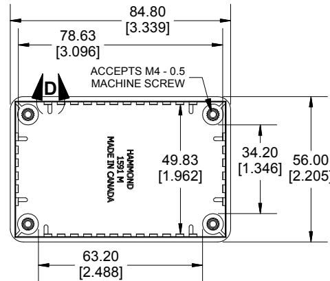
INSIDE BOX
