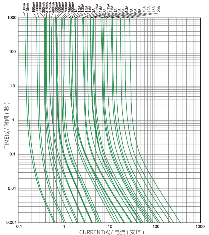
20N AVERAGE I-T CHARACTERISTICS CURVE (FOR REFERENCE ONLY) 20N 平均 I-T 曲线图 (仅供参考)
