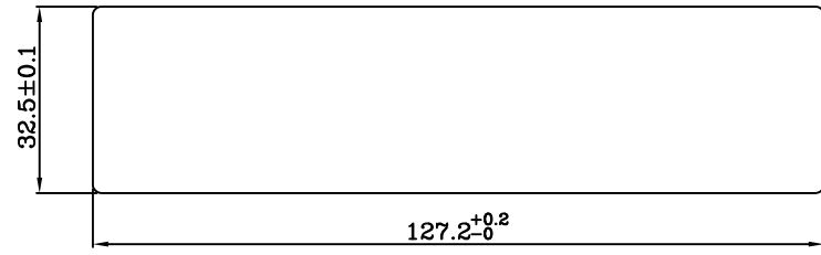
PANEL CUT-OUT
