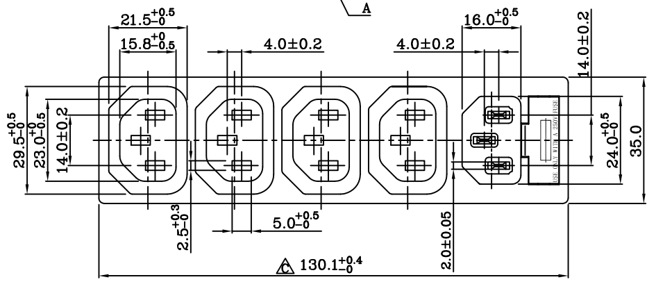
DRAWING:C:DG\NEW-R\T\3014\G24\R-3014G24 (07) XX. DWG
