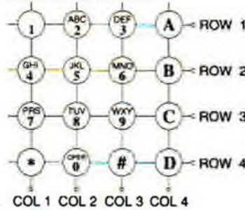
CIRCUIT DIAGRAM
