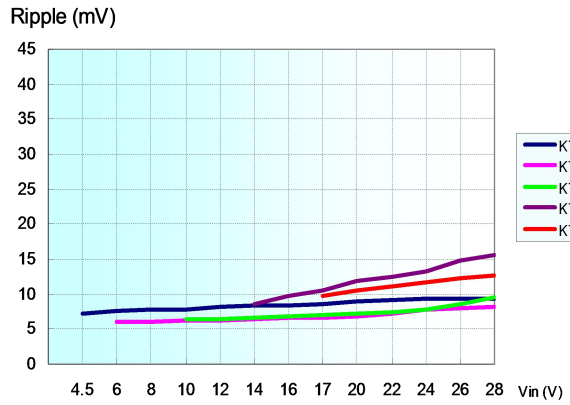
Ripple VS Vin ( Full Load)
