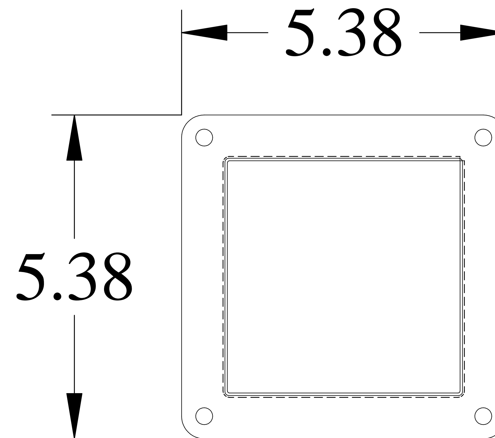
END VIEW
