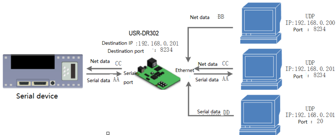
Diagram 4.2.3-1 UDP Client
