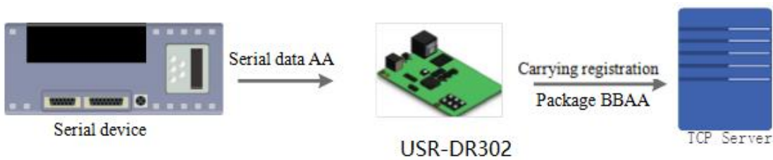
Diagram 4.8.2-1 Sending when establishing a connection
