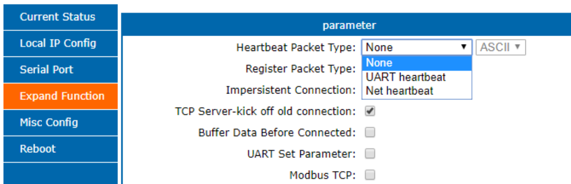
Diagram 4.8.1-2 Heartbeat Package
