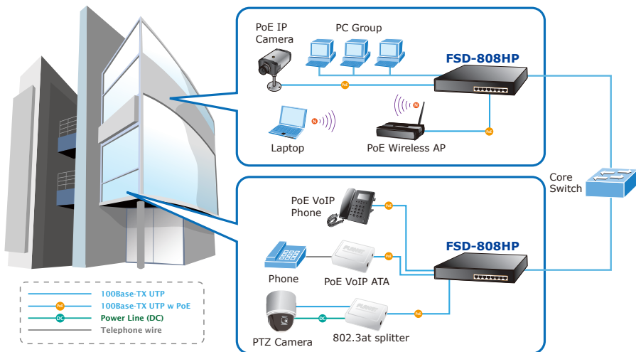
Figure 3-5: IP Office Department / Workgroup PoE Switch Connection
